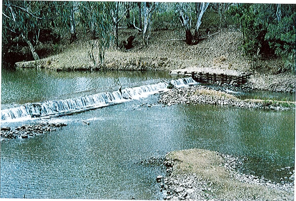
Photograph 9. The original wood-and-concrete weir at Goondiwindi on the Macintyre River before the construction of a rock-ramp in August 1993.
