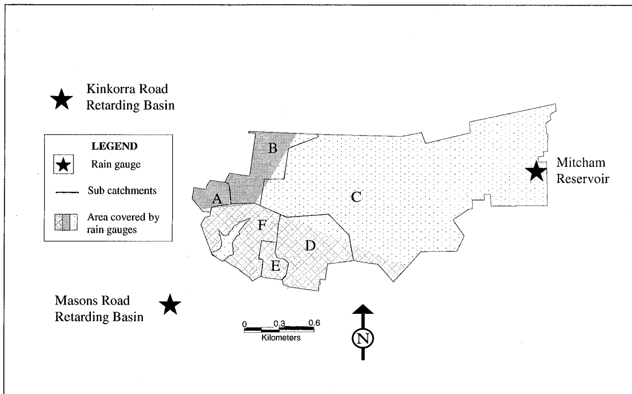
Figure 3.1 Rainfall station locations, and areas they cover using Thiessen polygons.
