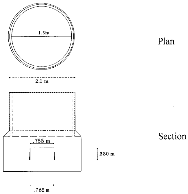
Figure 3.4 Glory hole structure at the outlet of the Lake.
