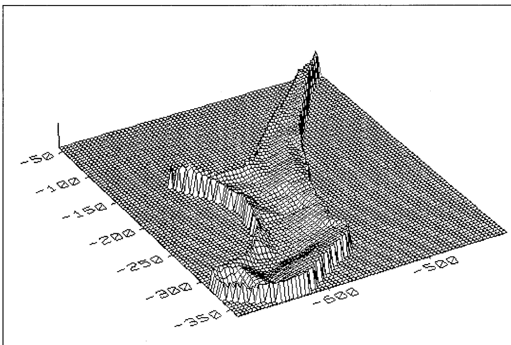
Figure 2.1 Results of Bathymetric survey of Blackburn Lake. Conducted by the CRCCH, April 1996.
