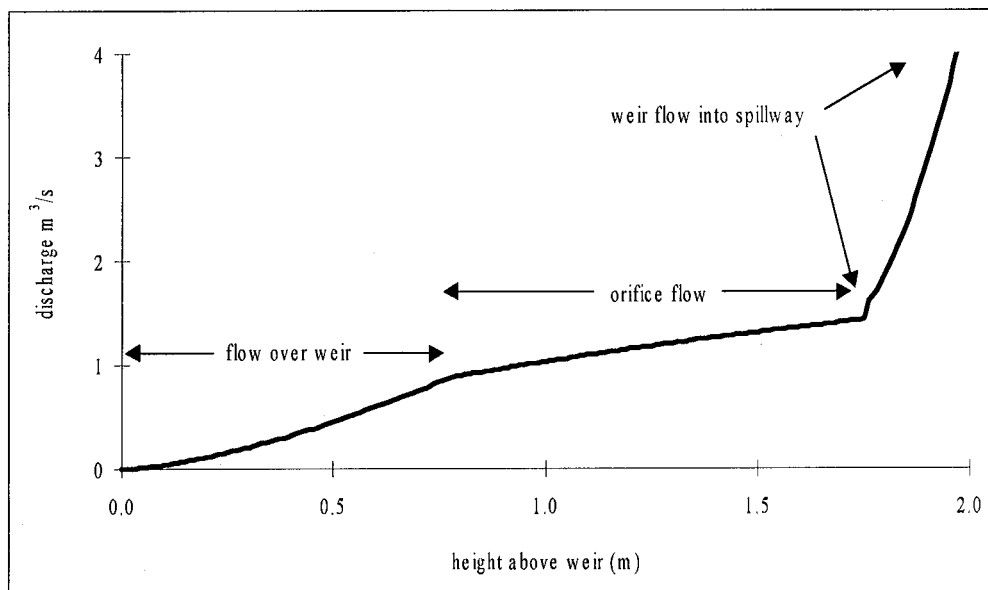
Figure 3.5 Stage discharge rating for outflow from Blackburn Lake.
