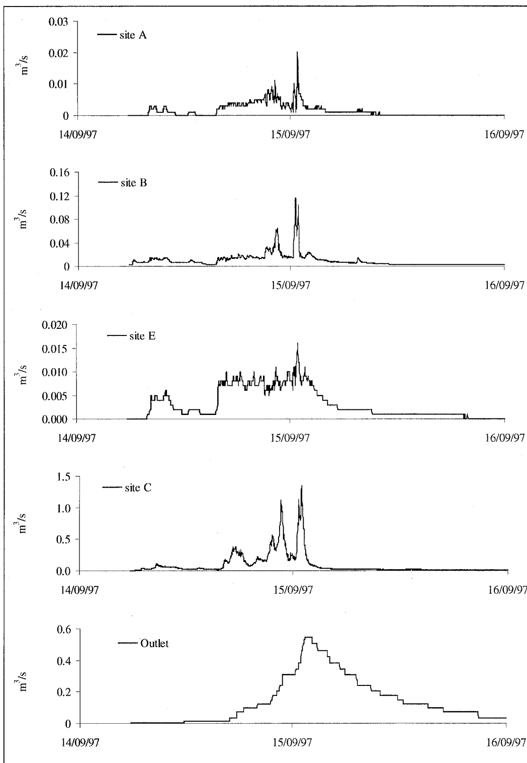
Figure 3.6 A typical event showing hydrographs for inflows to the lake from the sub catchments and the outflow from the lake.
