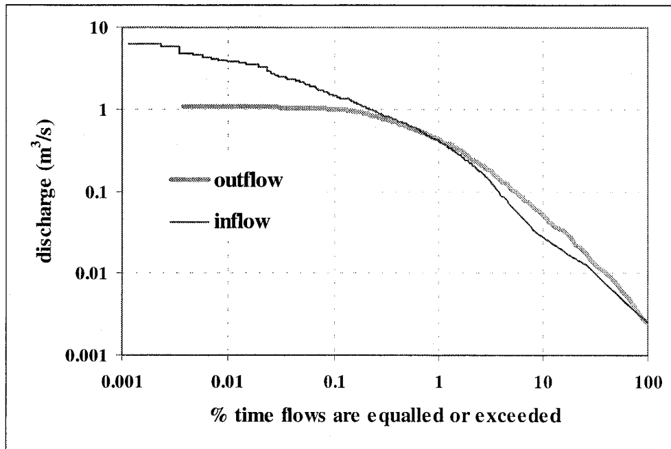
Figure 3.7 Flow duration curve for 2 years (1996 -1998) of inflow(C) and outflow from Blackburn Lake.
