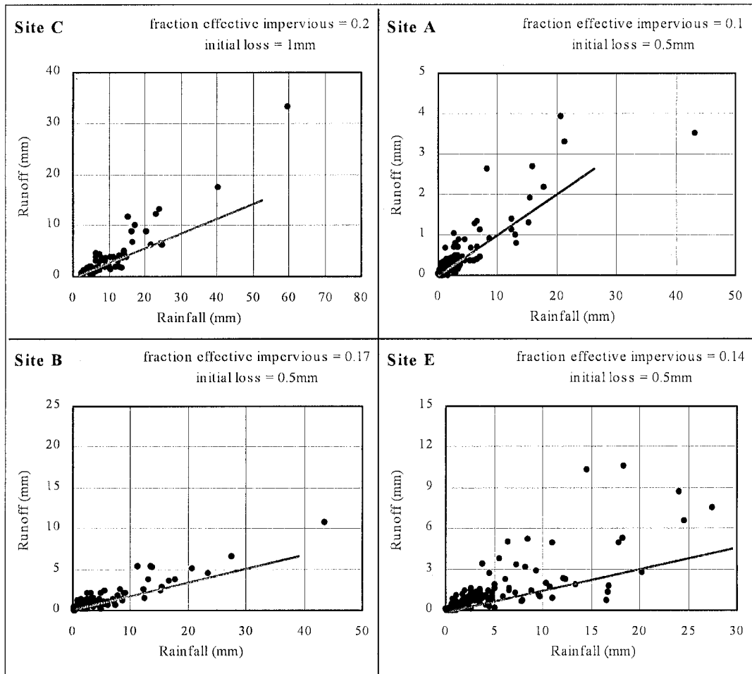
Figure B.2 Rainfall - runoff relationships for events for each site
