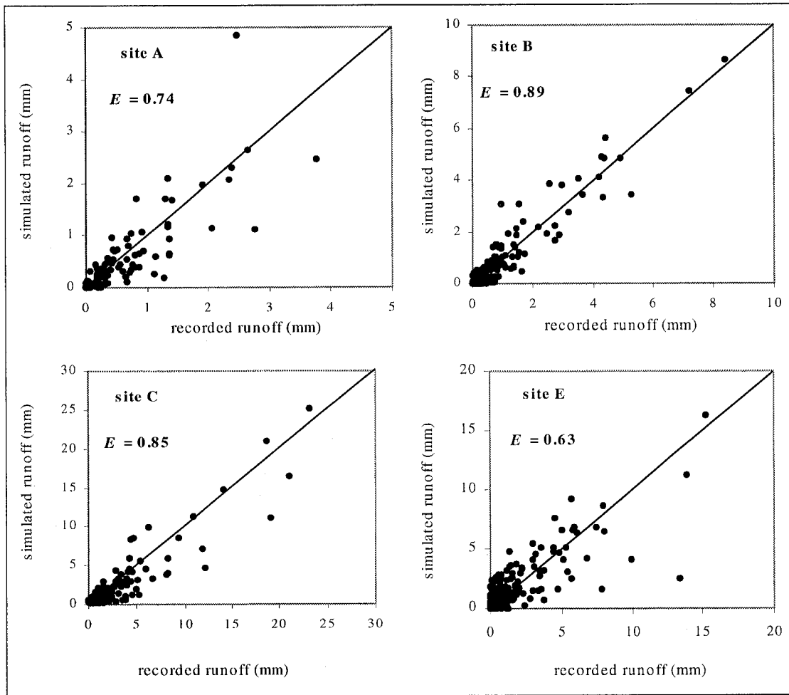
Figure 3.8 Modelled daily flows against measured flows
