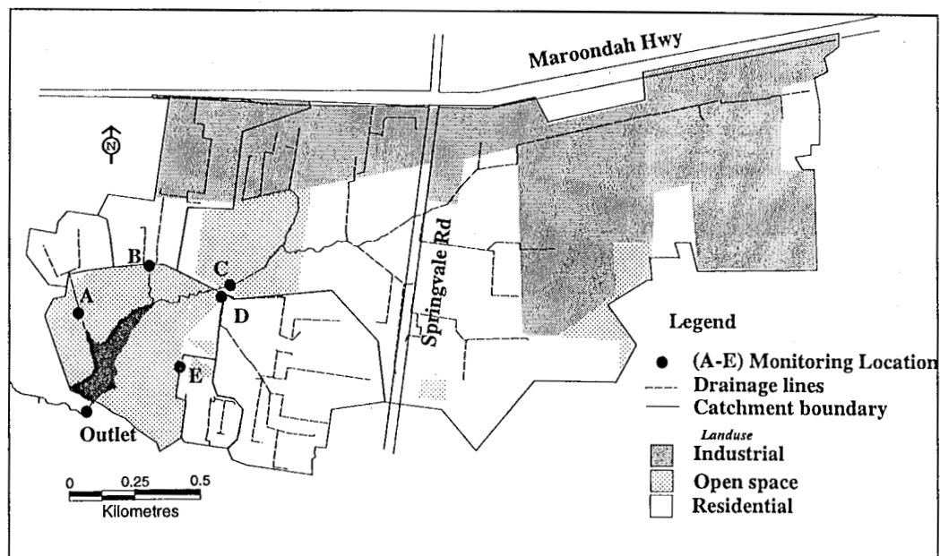
Figure 2.2 Blackburn Lake catchment boundary and monitoring site locations.
