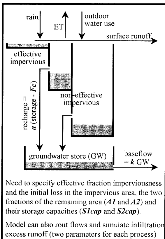
Figure B.1 Structure of daily runoff model
